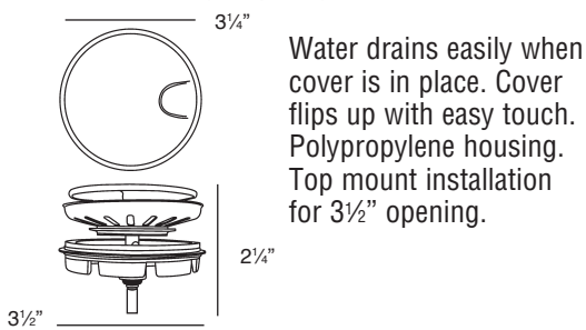
4010 Covered Flip Top Disposer Strainer.
